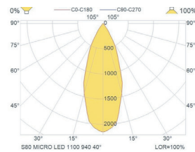
S80-MICRO-LED-1100-940-40
