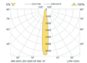
S80-MIDI-LED-4000-HF-930-15
