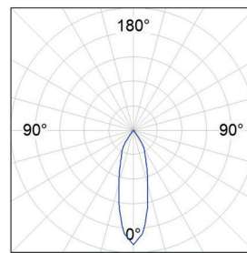
30° FLOOD
