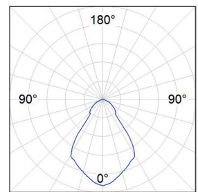
71° WIDE FLOOD
