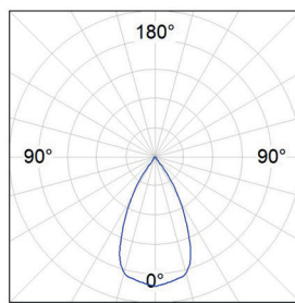
54° WIDE FLOOD
