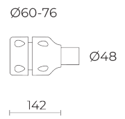
JOINT KIT
