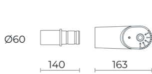
ADJUSTABLE JOINT
