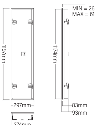
C64-R300X1200
