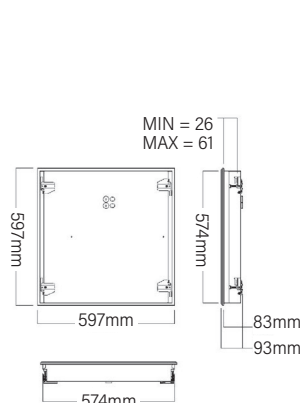
C64-R600X600
